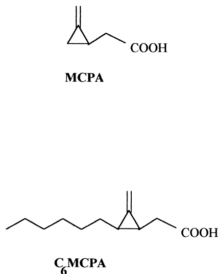
Fig. 1. Structure of the free acid forms of MCPA and C 6 MCPA.
